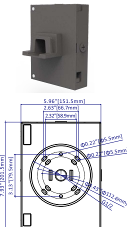
Wall Mount
