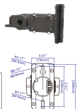
Universal bracket
