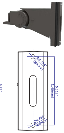
Adjustable Square & Round Pole Mount
